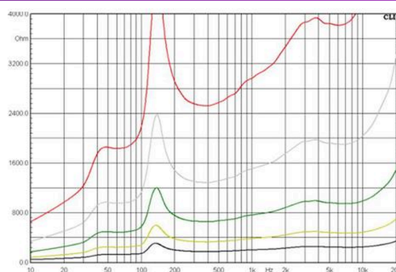
Impedance vs Frequency (all taps)
