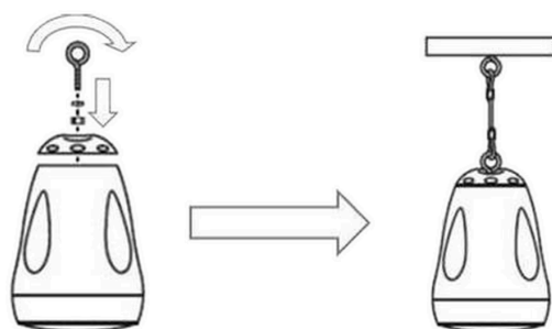
1. Fit the eyebolt to the speaker top
