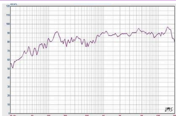
SPL vs Frequency
